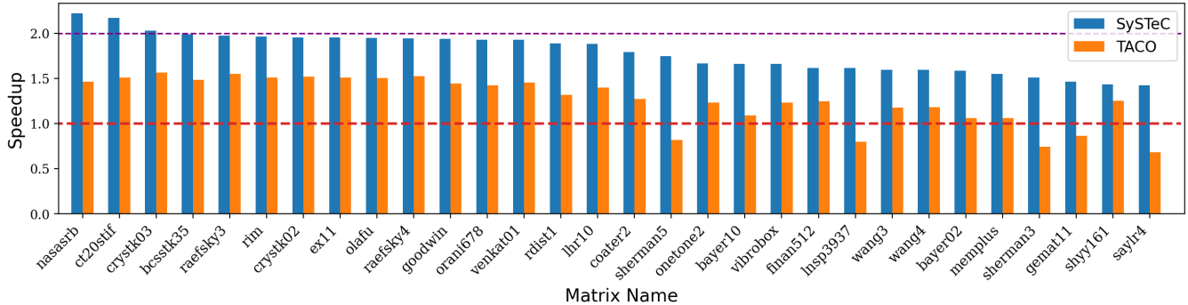
Figure 8. SYPRD Performance
