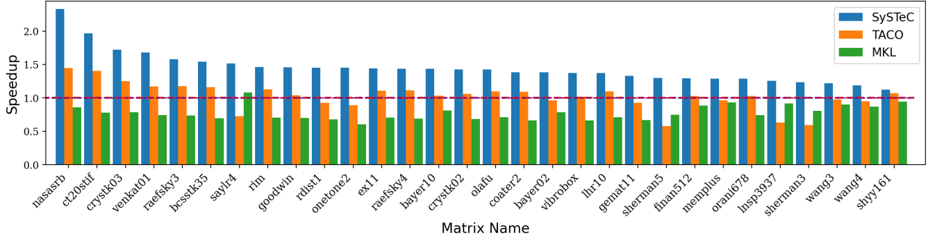
Figure 6. SSYMV Performance
